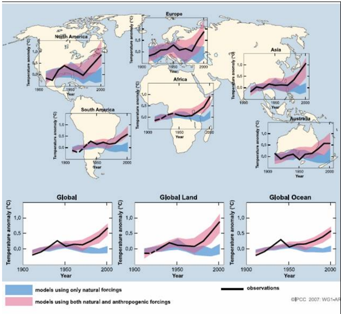
Figure 3.1: Identifying the signal of anthropogenic warming on continental scales
