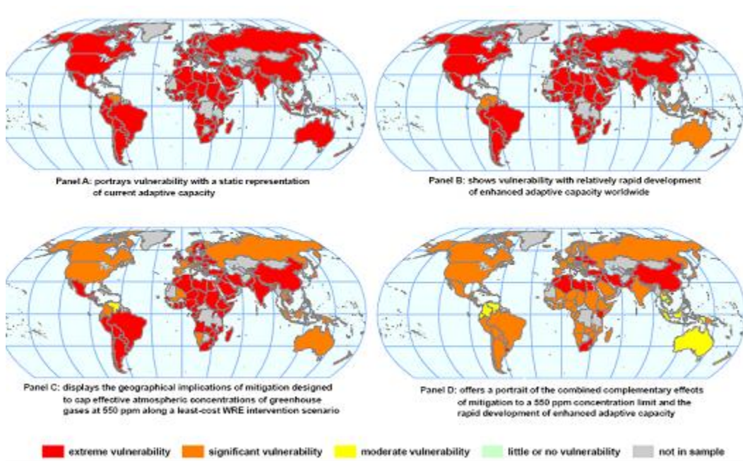
Figure 3.7: Geographical Distribution of Vulnerability in 2050 (A2 emissions; high climate sensitivity)
