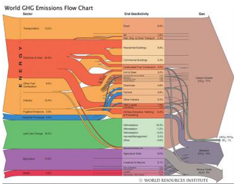
Figure 6.1: A Flow Chart of World GHG Emissions
