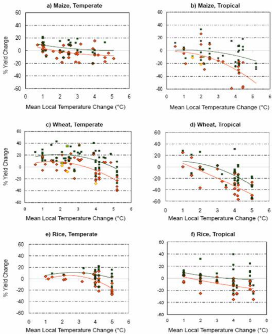
Figure 3.5: Sensitivity of crop yields to changes in local temperature with and without adaptation
