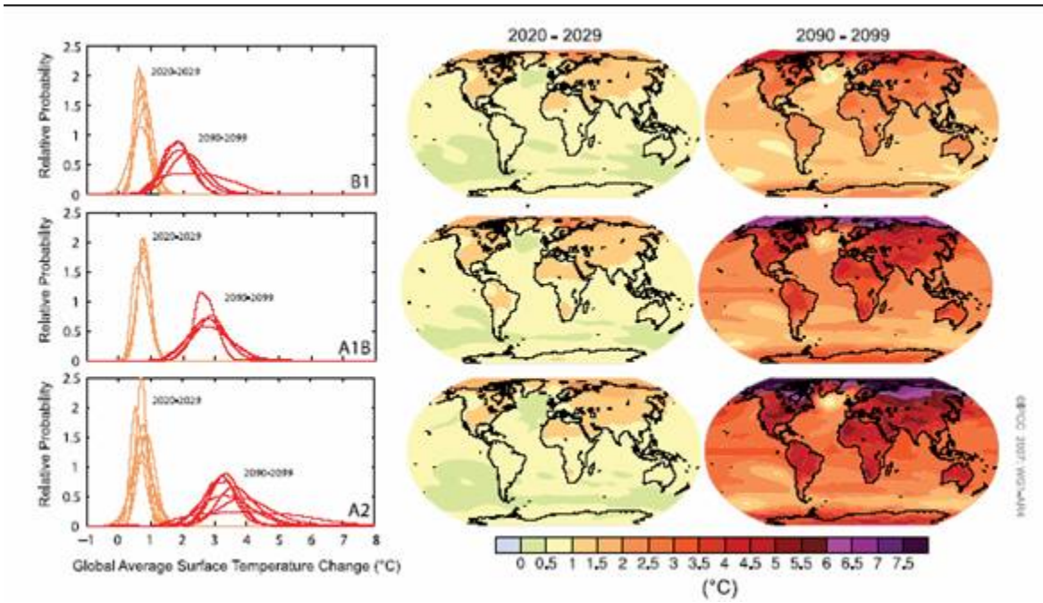
Figure 3.2: Projections of surface temperatures for the 2020's and the 2090's.
