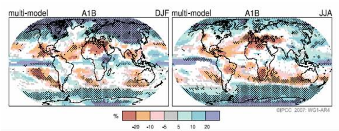
Figure 3.3: Projected changes in precipitation patterns across the globe in the 2090's
